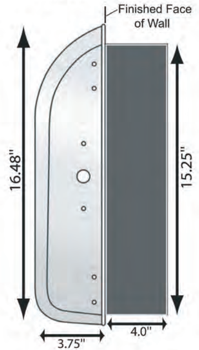
SIDE EXTERIOR
